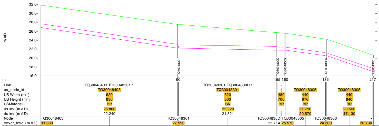
Figure 4: Example 1 as original Sewer Records
