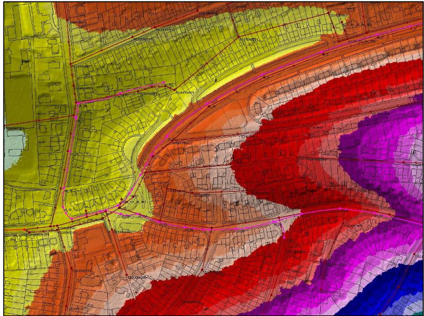
Figure 13 : DTM with overland flow routes identified
