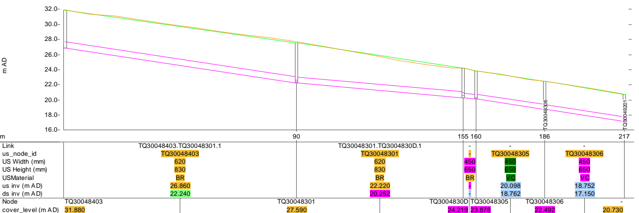
Figure 6: Example 1 with corrected Sewer Records
