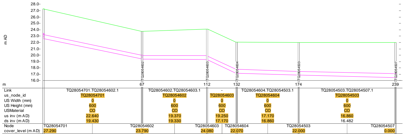
Figure 7: Example 2 showing original Sewer Records
