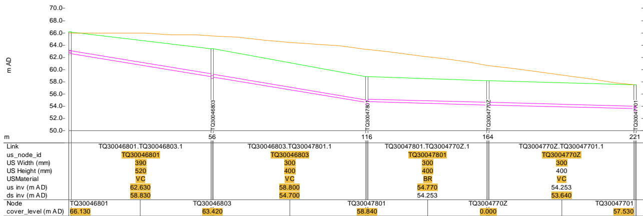
Figure 10 : Example 3 as original Sewer Records but also showing the DTM
