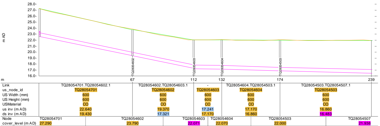
Figure 9 : Example 2 showing corrected Sewer Records
