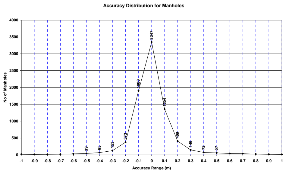
Figure 3 : Distribution of Manhole Cover Levels compared to DTM
