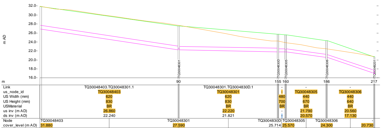
Figure 5: Example 1 with DTM on original Sewer Records
