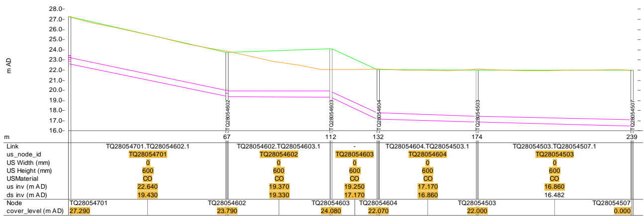
Figure 8 : Example 2 with DTM overlying original Sewer Records
